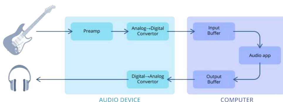
Audio processing (simplified)
