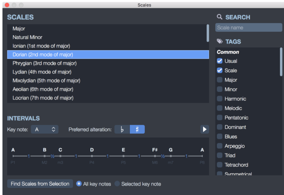
Scales library
